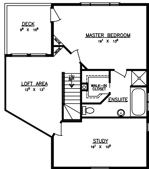
SECOND FLOOR AREA = 822 S.F.
